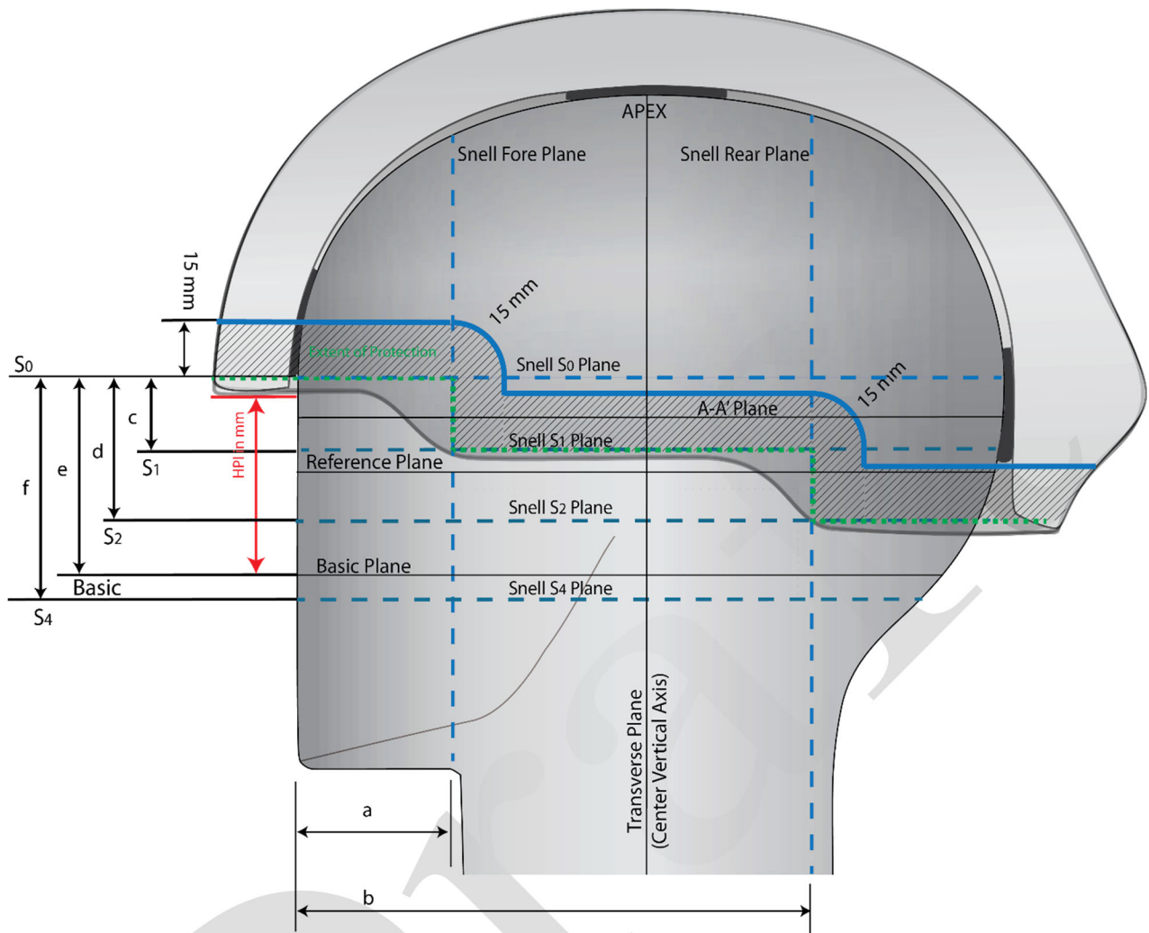
ISO DIS 6220-1983/EN960 Head Form
