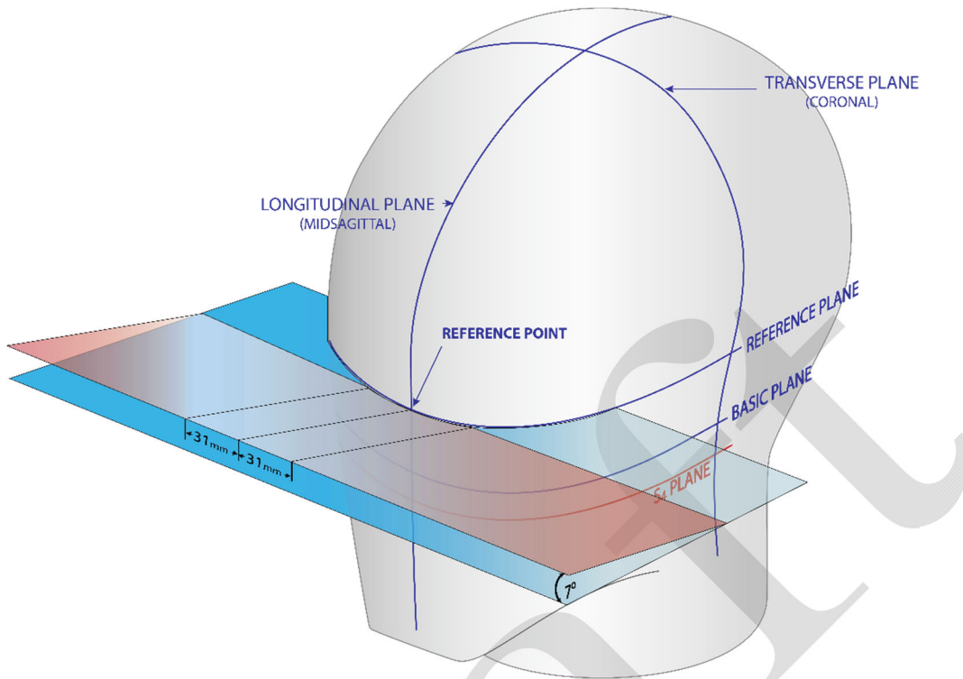
Figure 3. Upward Visual Clearance
