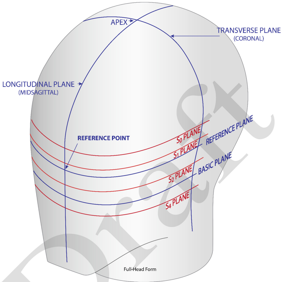
Figure 1 - ISO Head Form – ISO DIS 6220-1983
